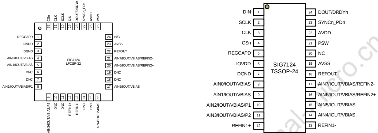
TOP VIEW (Not To Scale)
